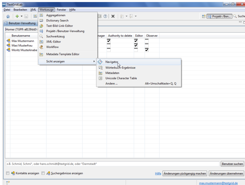
Figure 2: Open Navigator
